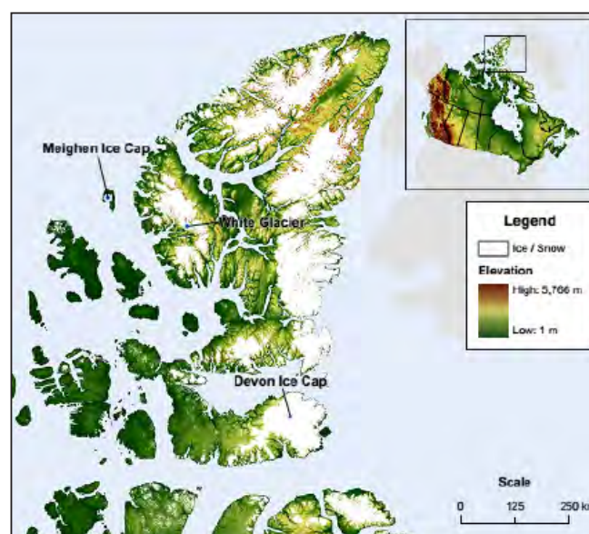
Figure 29. High Arctic glaciers
