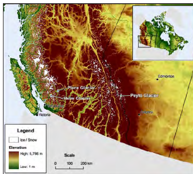
Figure 30. Western Cordillera glaciers
