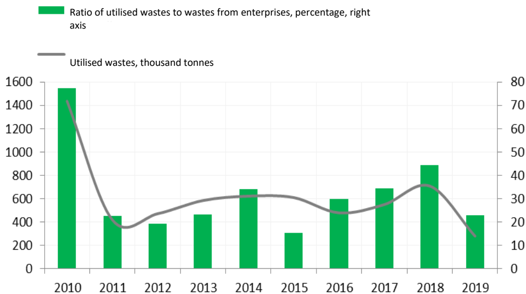
Figure 27. Recycled waste, and the ratio between recycled waste and waste generated by enterprises
