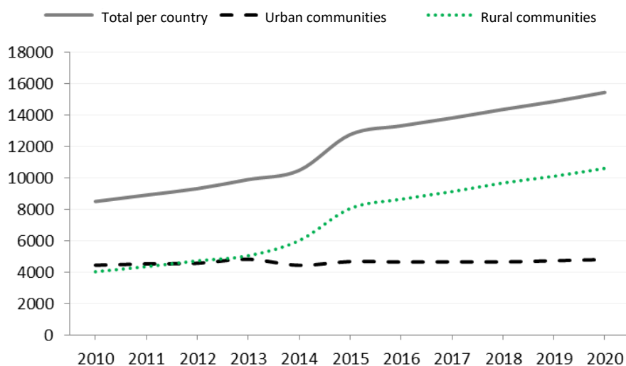
Figure 44. Public water supply networks length (km)
