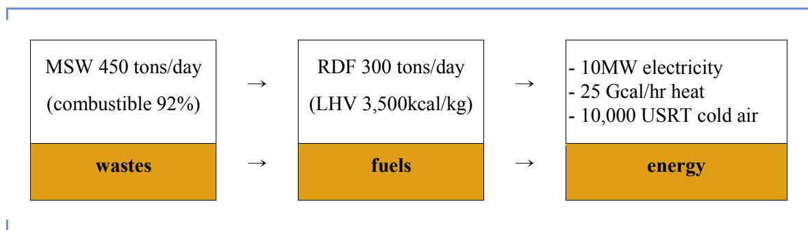
Figure IV-6 | Waste-to-Energy Planst Process
