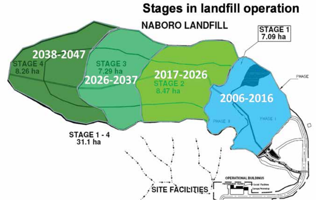
Figure 70. A plan showing the duration of different stages of landfill operation and hectares of area required for each stage. 190
