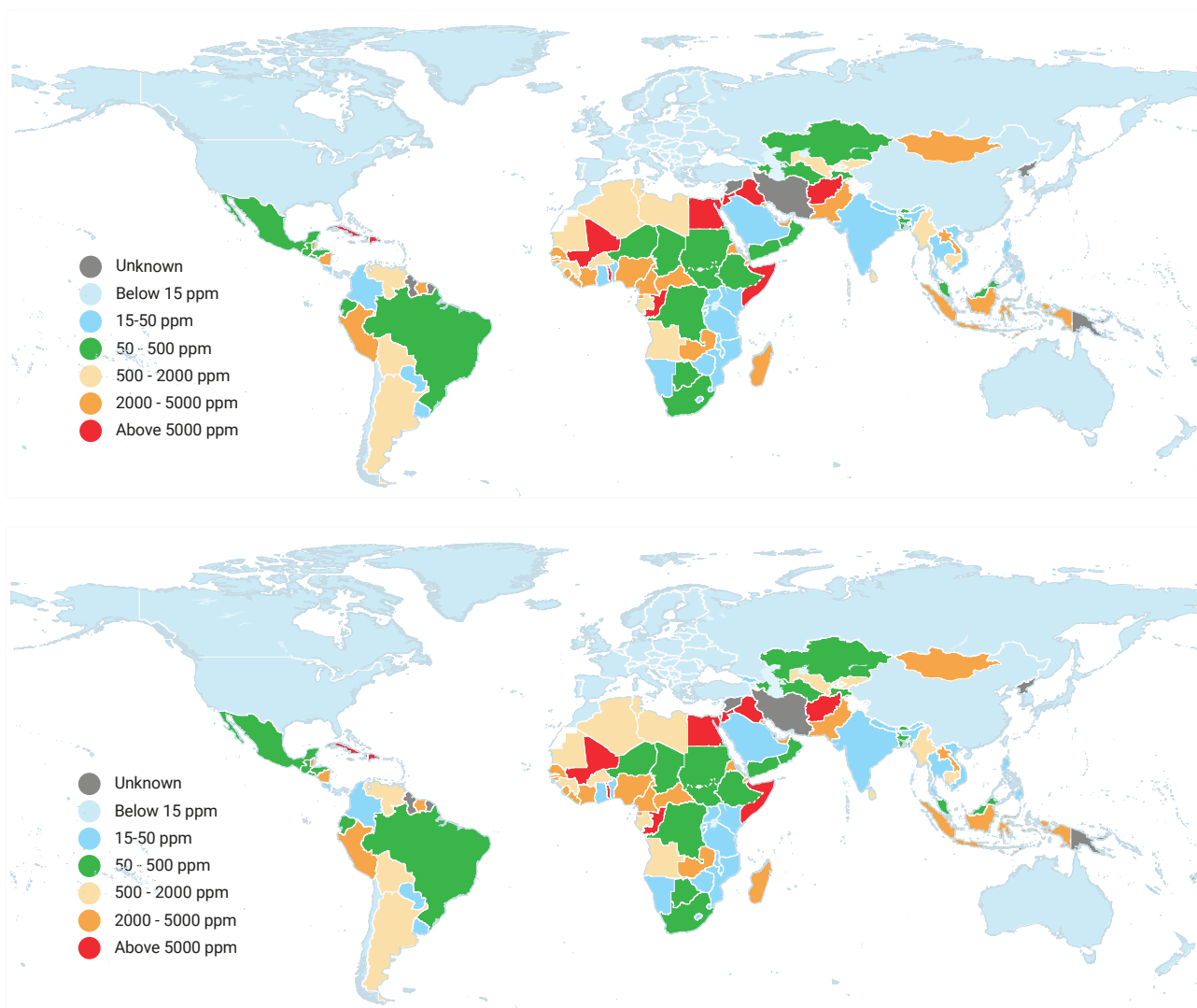
Figure 14. Map of maximum allowed diesel sulphur content in 2016 (Top) and 2020 (Bottom)
