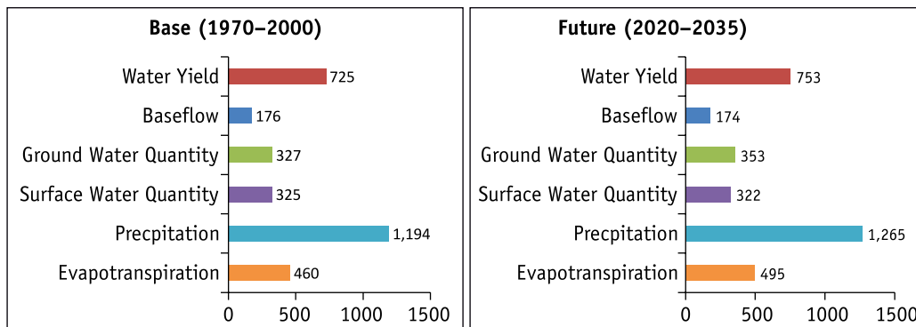
Figure 3.12: WBC of Chenab sub-basin
