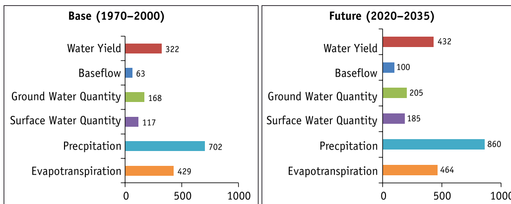
Figure 3.11: WBC of Ravi sub-basin
