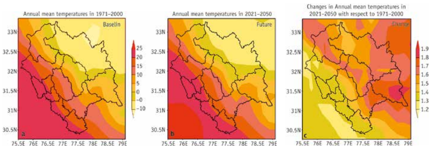
Figure 2.15: Mean annual temperature for baseline period (a), near future (b), and change in near future (c) relative to baseline period
