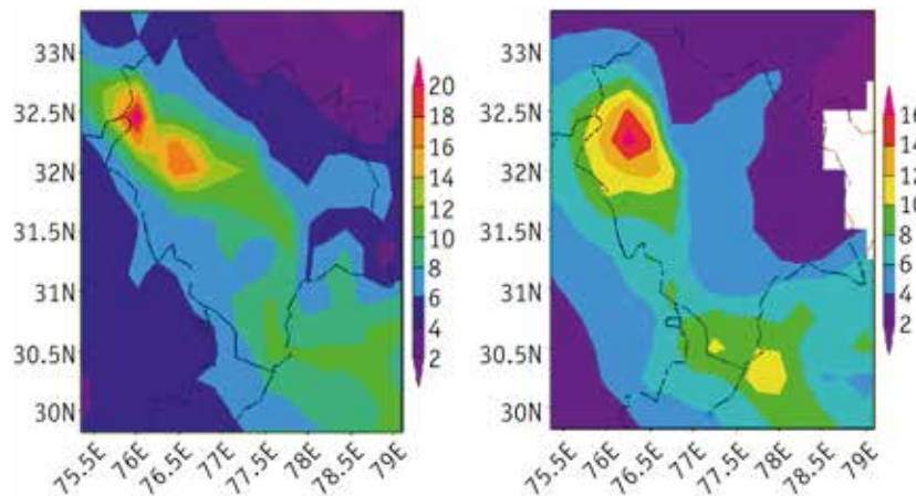
Figure 2.9: Monsoon (JJAS) rainfall climatology from IMD (left) and PRECIS (right) for the baseline period 1970–2000, both showing a high rainfall zone in the north
