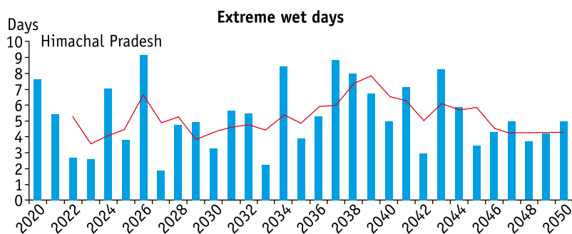
Figure 2.19: Extreme Wet days in future relative to extreme rainfall in baseline
