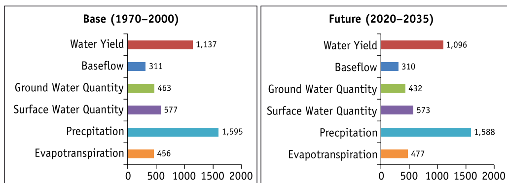
Figure 3.14: WBC of Sutlej Upper sub-basin
