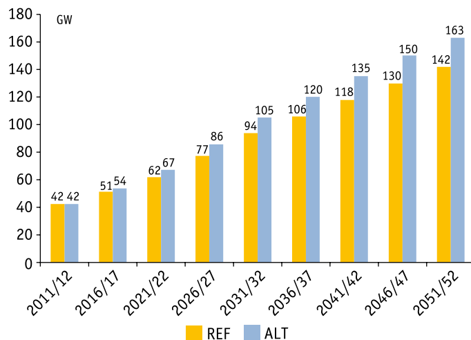
Figure 4.3: Hydropower generation capacity (in GW) for India under different scenarios
