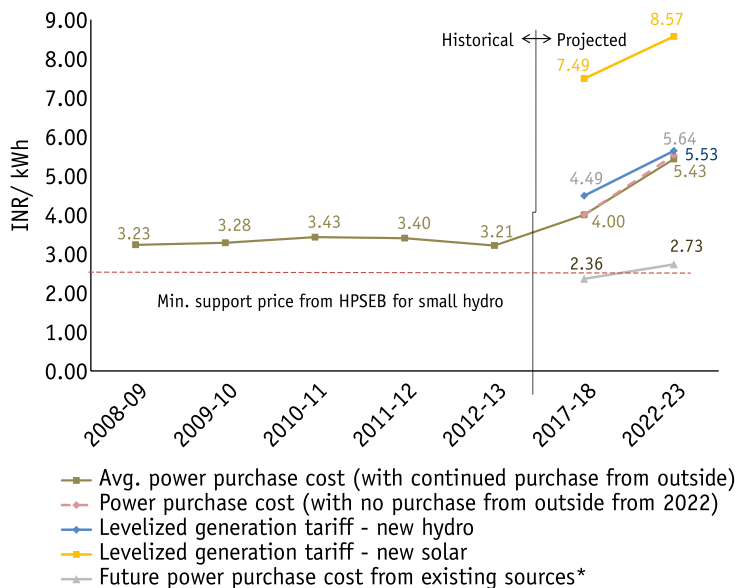
Figure 4.11: Projected power purchase cost in Himachal Pradesh (2017–22)
