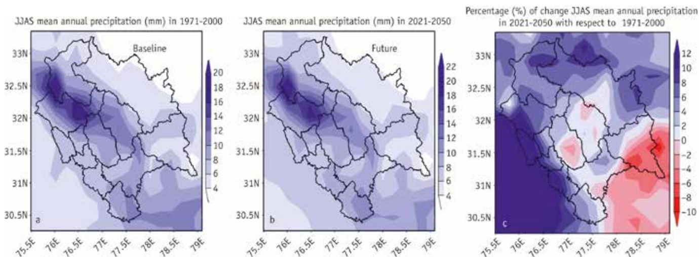
Figure 2.11: Mean annual summer monsoon precipitation for baseline period (a), near future (b), and change in near future (c) relative to baseline period
