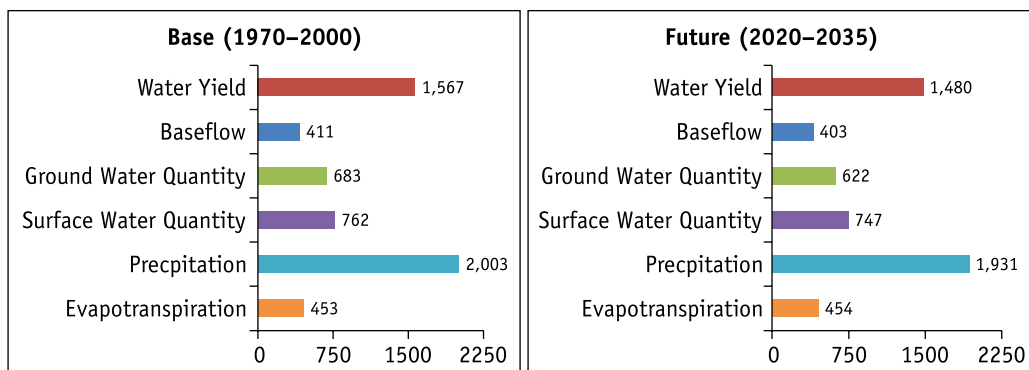
Figure 3.13: WBC of Upper Indus sub-basin
