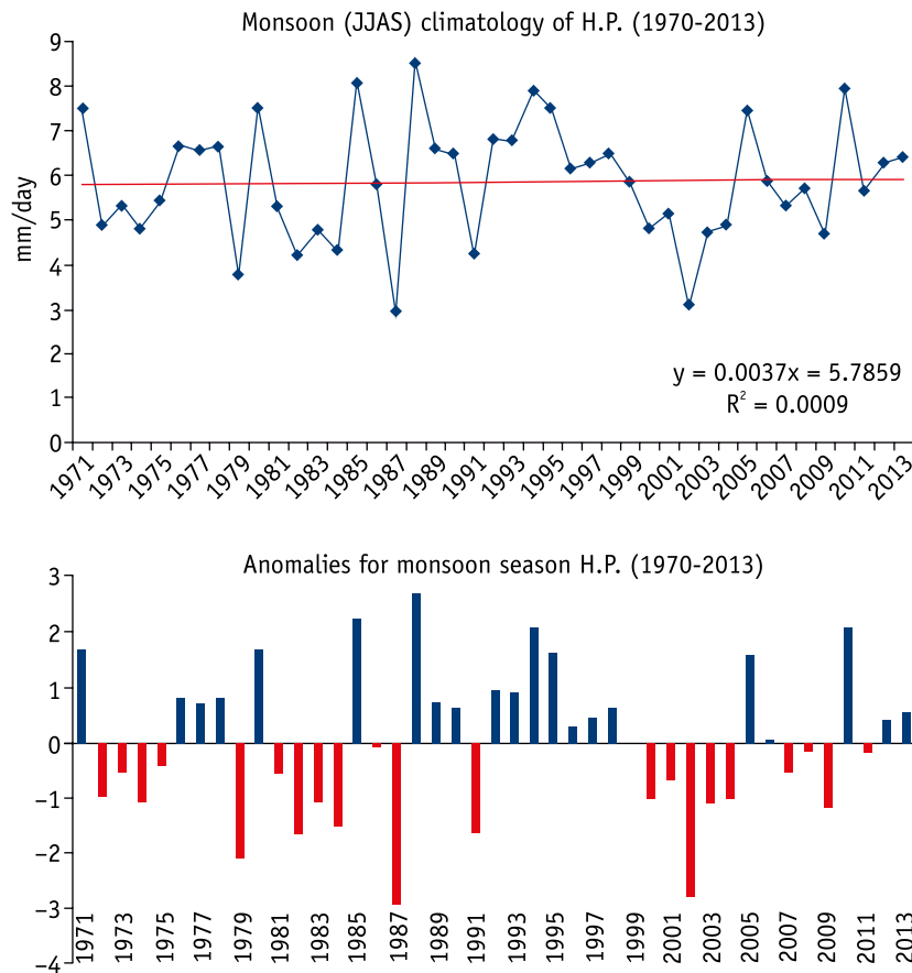
Figure 2.8: JJAS rainfall (a) climatology and (b) anomaly over Himachal Pradesh for the 1970–2013 period
