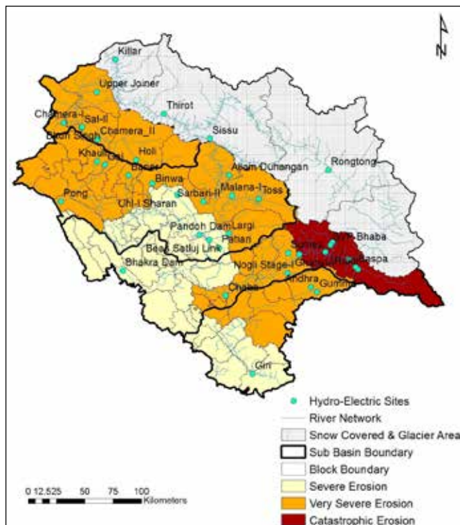
Figure 3.17: HEP regions affected due to soil erosion by water (2030s)
