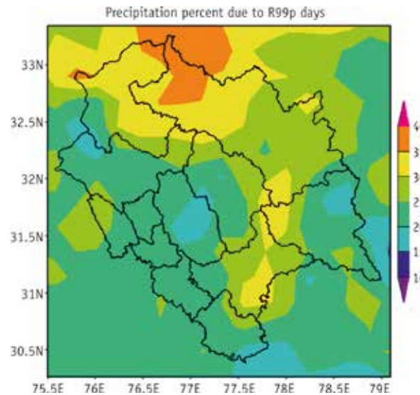
Figure 2.18: Extreme wet days contribution to the total rainfall—near future
