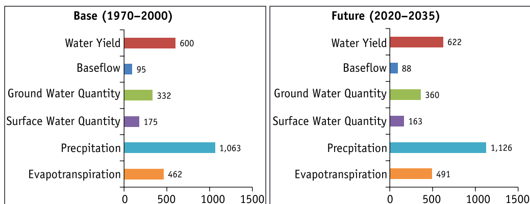
Figure 3.15: WBC of Yamuna Upper sub-basin
