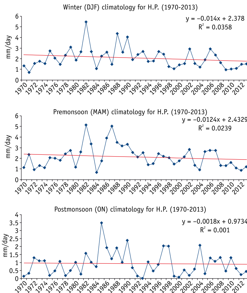
Figure 2.7: Rainfall climatologies for Himachal for (a) winters, (b) pre-monsoon, and (c) post-monsoon for the 1970–2013 period Source: TERI Analysis
