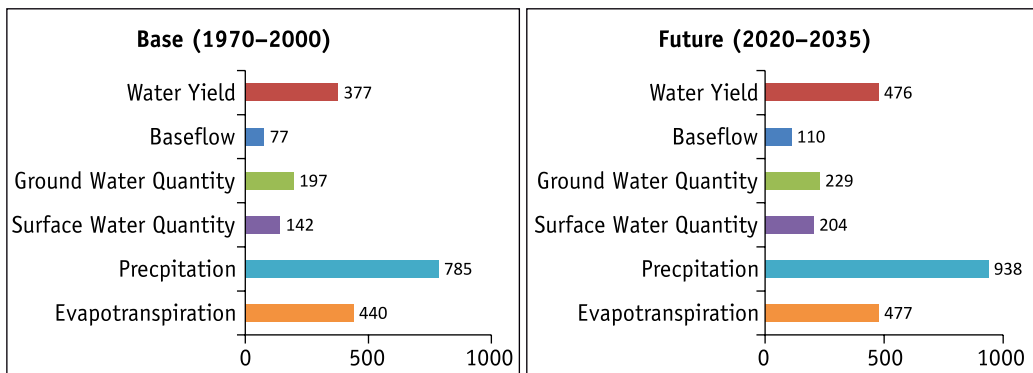
Figure 3.10: Water balance components (WBC) of Beas sub-basin
