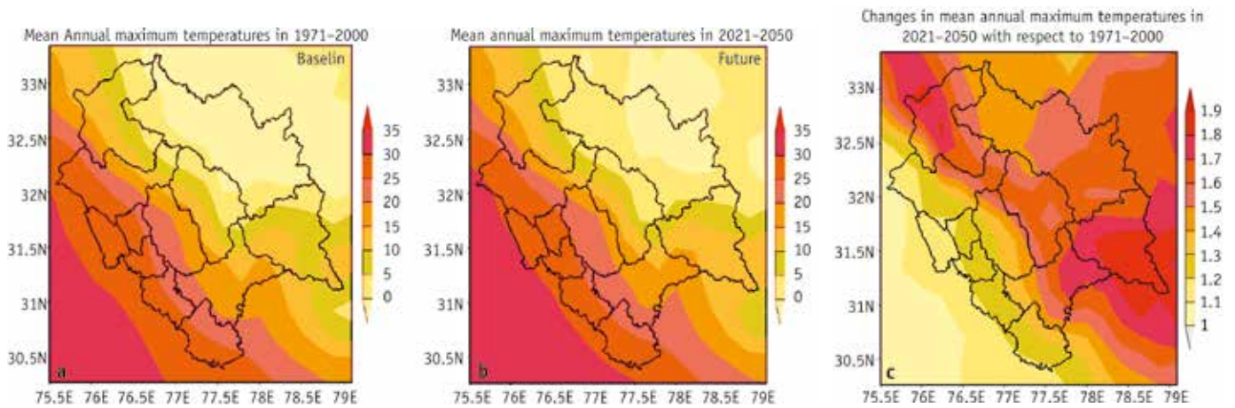
Figure 2.16: Mean annual maximum temperature ( T_{max} )
