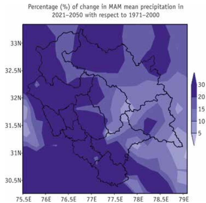
Figure 2.13: Mean summer precipitation change for near future (2020–2050) relative to 1970–2000
