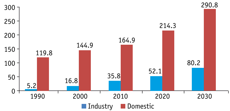
Figure 3.2: Industrial and domestic water requirement (1990–2030) in million meter cube
