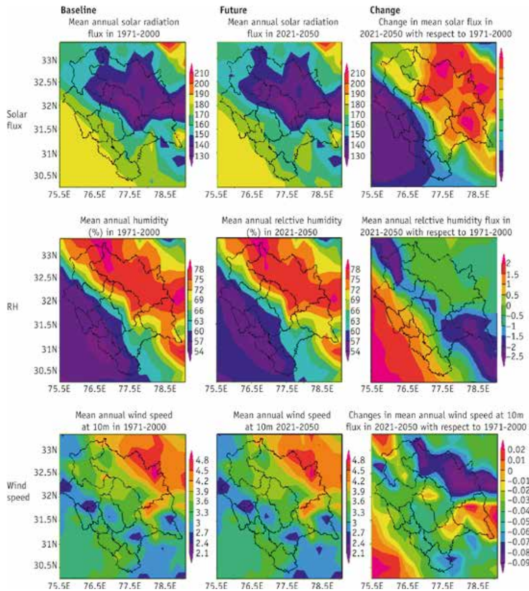
Figure 2.20: Spatial pattern of solar flux (top panel), relative humidity (middle panel), and wind speed (bottom panel) and the change in near future relative to the baseline period.
