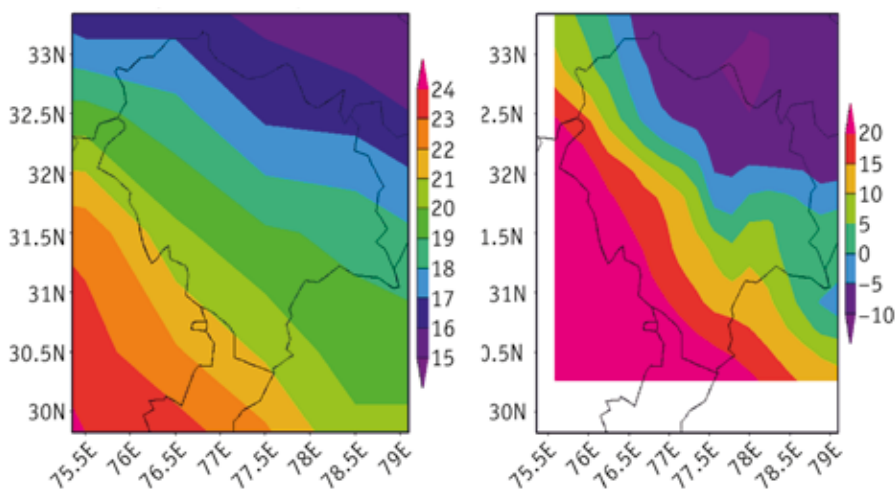
Figure 2.10: Annual mean temperatures from IMD (left) and model (right) for 1970–2000 baseline period over Himachal Pradesh
