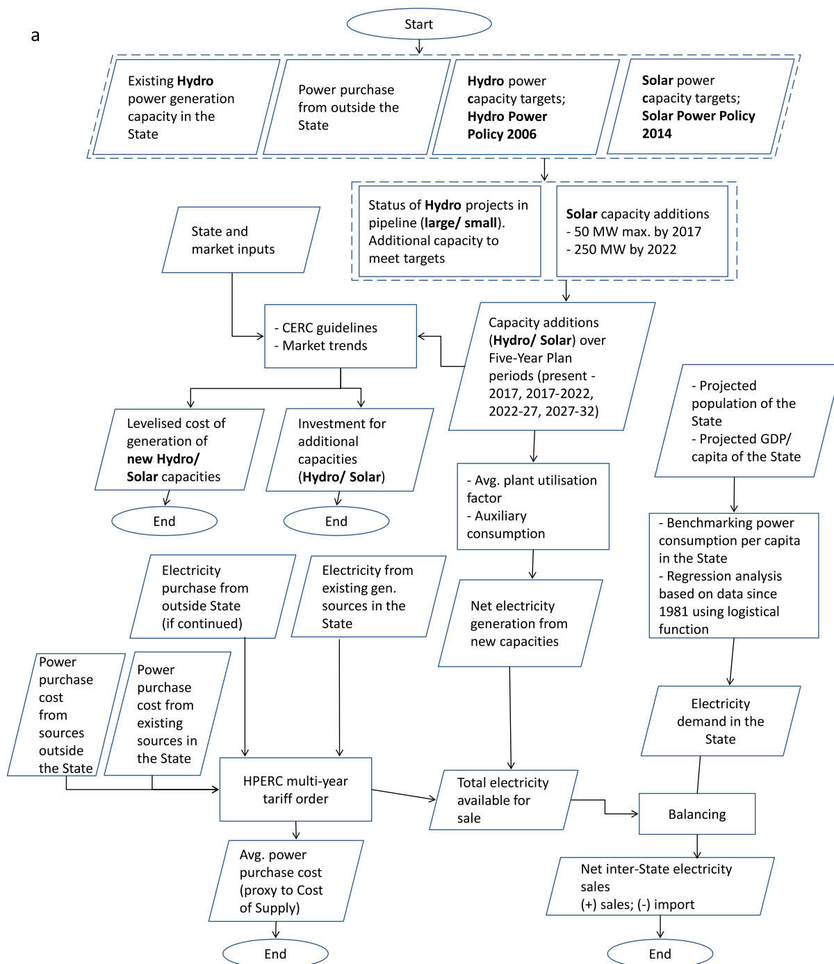
Figure 4.7: Schematic representation of the modelling projection methodology
