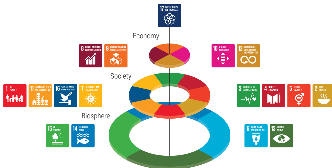
Figure 2.7: The three dimensions of sustainability (adapted from Stockholm Resilience Centre 2016)
