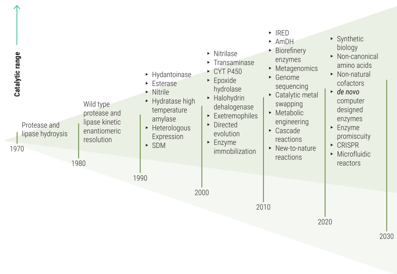
Figure 4.5: Scope of Biocatalysis in Sustainable Organic Synthesis (Sheldon and Brady 2019, p. 2859)
