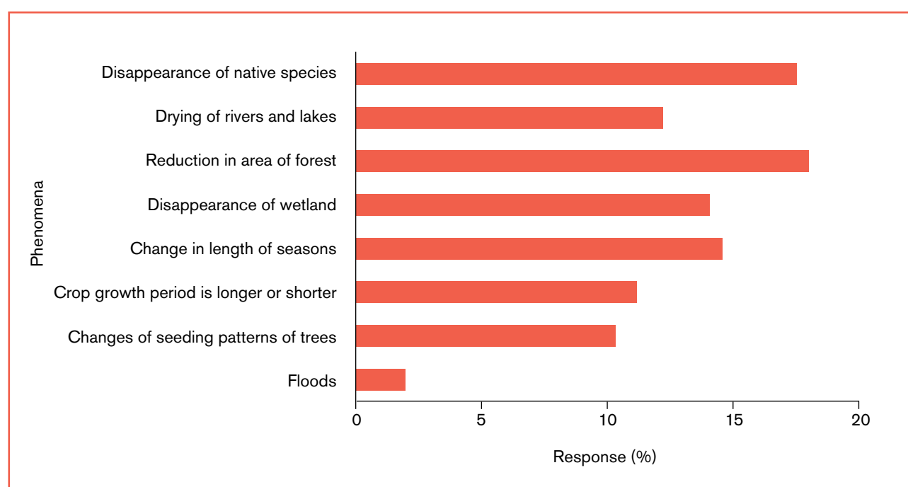
Figure 19: Ecological changes (phenomena) associated with climatic changes observed
