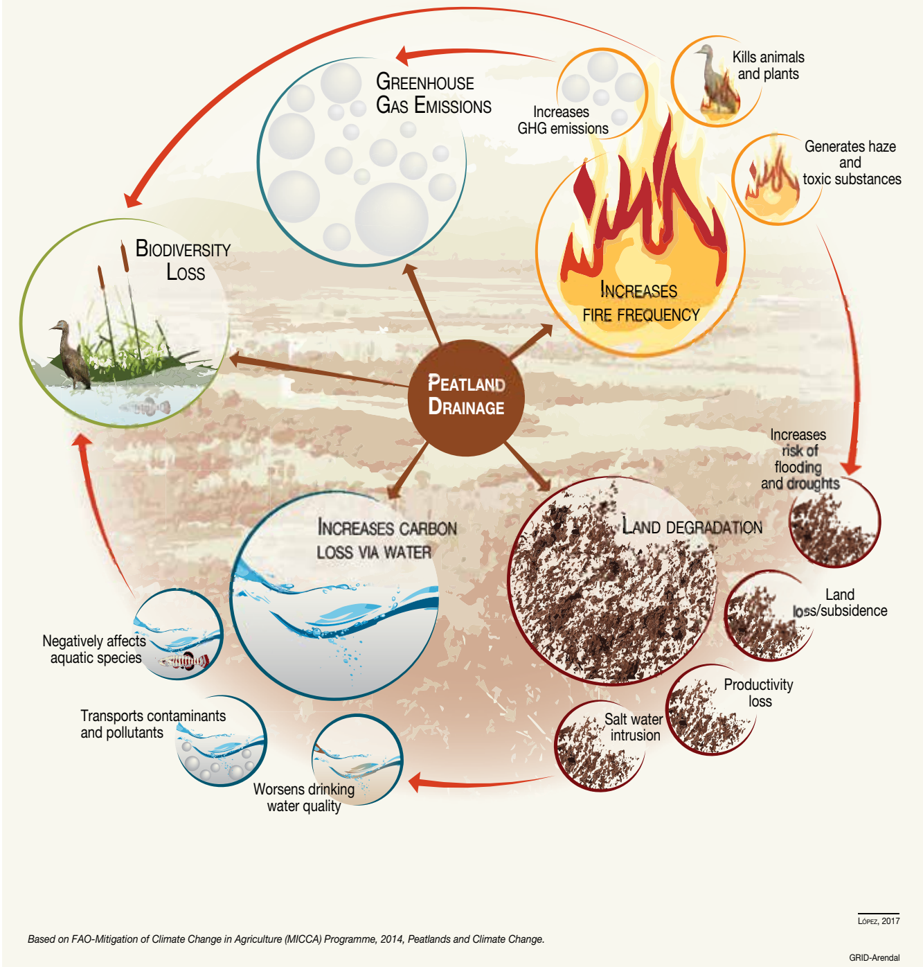
Figure 9. An illustration of the environmental and social effects of peatland drainage.
