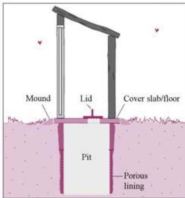
FIGURE 5-1 PIT LATRINE - TYPICAL DESIGN
