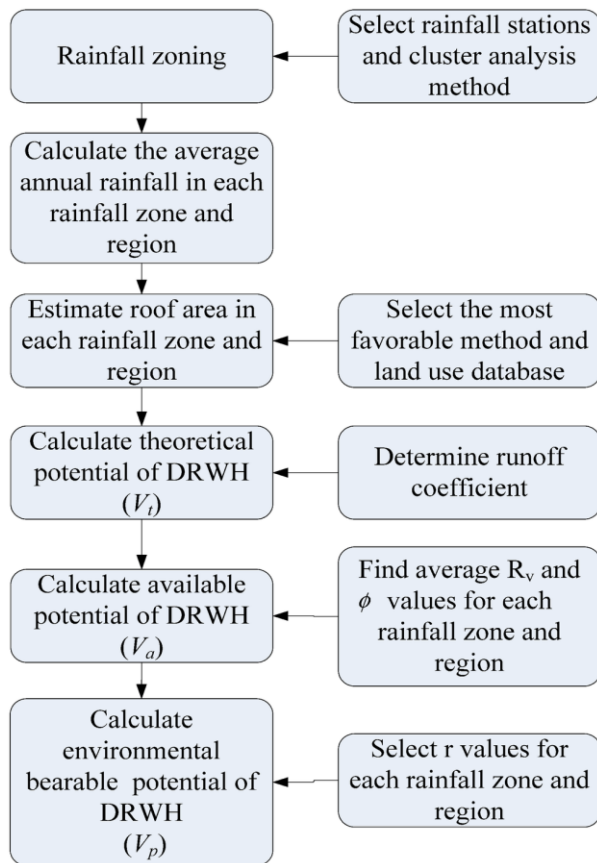
FIGURE 3-3 STEP BY STEP PROCESS FOR DESIGNING DOMESTIC RAINWATER HARVESTING (DRWH) RUN-OFF
