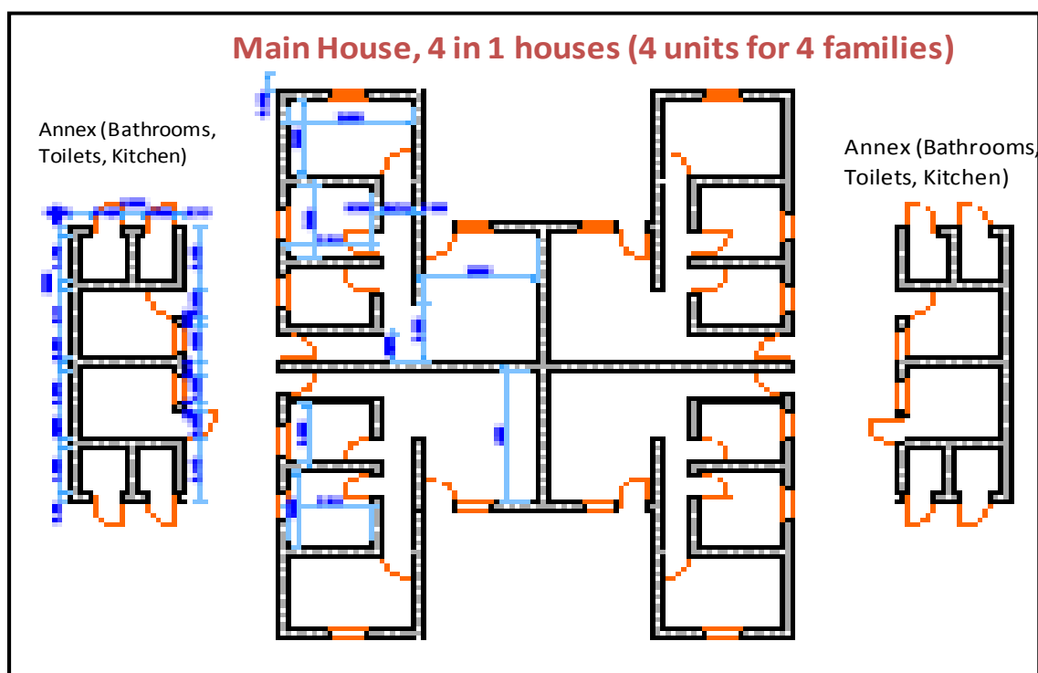
FIGURE 6-7: SEMI-DETACHED HOUSES 4 IN 1 - PROPOSED DESIGN PLOT SIZE IS 25 M X 20 M
